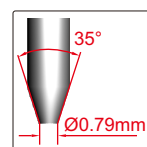
blunt taper indenter
